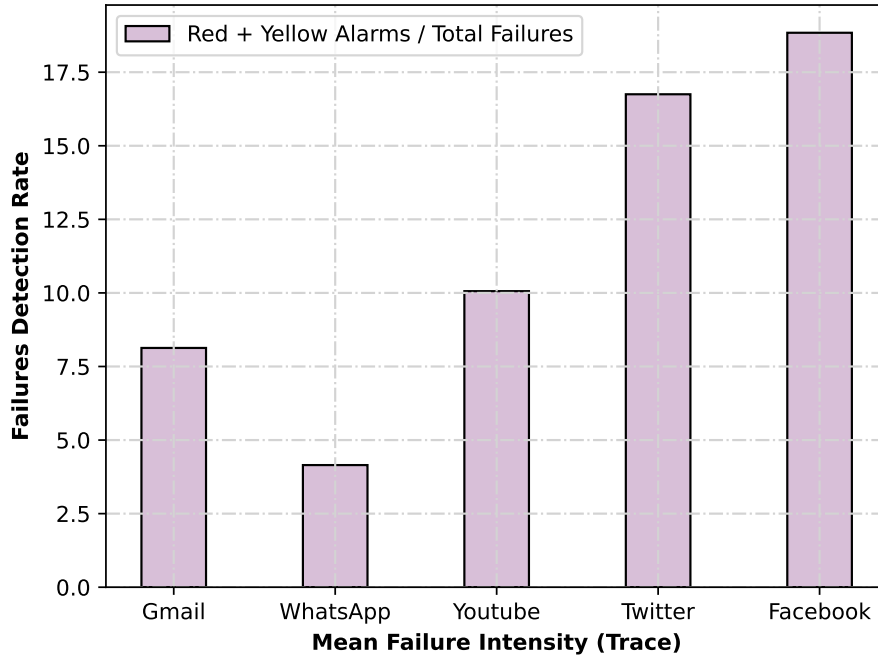
Figure 5.4: In this figure we show the total failure detection rate (■ Red + Yellow Alarms / Total Failures). Our results are much different from DyTwin’s performance [15]. We believe this is due to the irreconcilable differences between our experimental setups.
