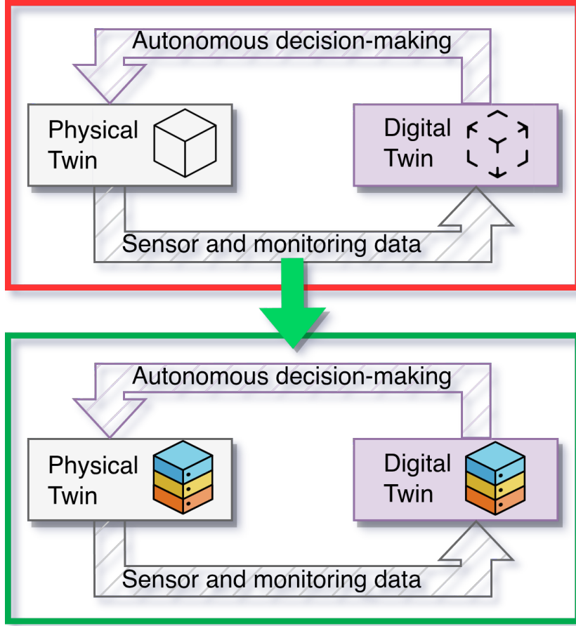
Figure 5.1: A novel evaluation method which solves the issue of real-world experimentation, which is unsustainable and costly [18].
