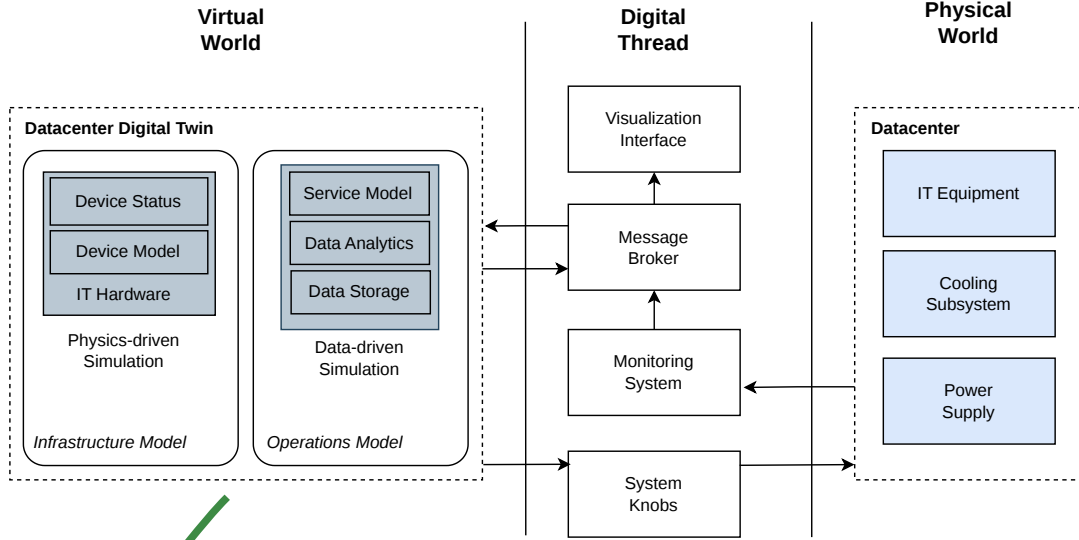
Figure 2.3 A generic system model for datacenter digital twin deployments. The design of DyTwin [37] indirectly incorporates in its architecture a “virtual-to-virtual” digital thread between different digital twins. Zhao et al. likewise present key elements to the digital thread in their architecture [42]. We add the Digital Thread to our model explicitly.
