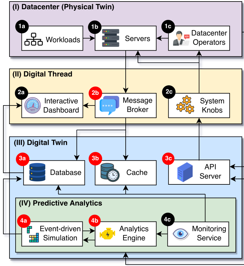
Figure 3.1 The predictive datacenter digital twin reference architecture. We call the system Sunfish . The architecture was designed with the AtLarge Design Process [14] over several iterations in the past months.
