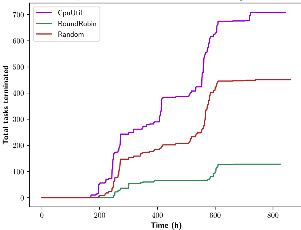
Comparison of Different Victim Selector Algorithms
