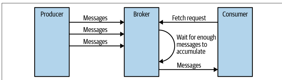
Figure 6-3. Broker delaying response until enough data accumulated
