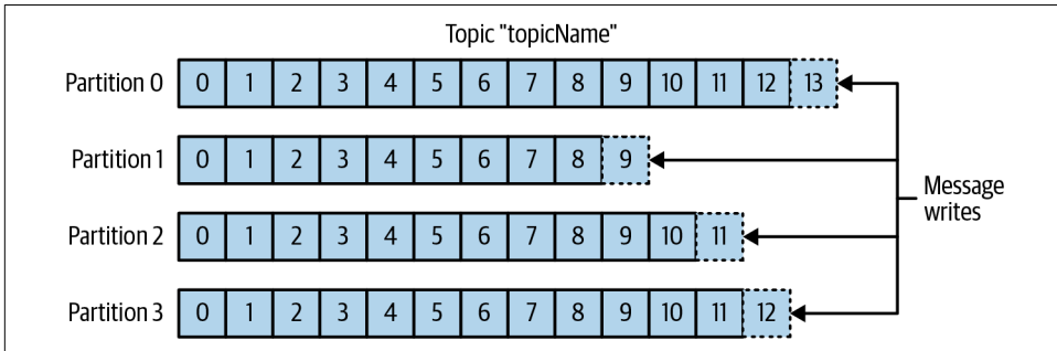
Figure 1-5. Representation of a topic with multiple partitions
