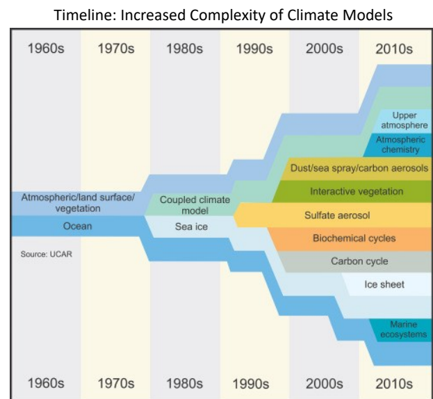
FIGURE 1 Hierarchy of temporal and spatial scales ( left ) and timeline of model complexities ( right ). SOURCE: Christiane Jablonowski, University of Michigan, presentation to the workshop. Left : Modified from The COMET Program (the source of this material is the COMET® website at http://meted.ucar.edu of the University Corporation for Atmospheric Research, sponsored in part through cooperative agreements with the National Oceanic and Atmospheric Administration and the Department of Commerce; © 1997–2023 University Corporation for Atmospheric Research; all rights reserved). Right : Copyright University Corporation for Atmospheric Research, licensed under CC BY-NC 4.0 License, via OpenSky.
