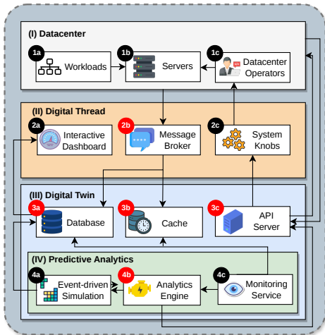
Figure 1.4: The predictive datacenter digital twin reference architecture. The architecture was designed with the AtLarge Design Process [7].
