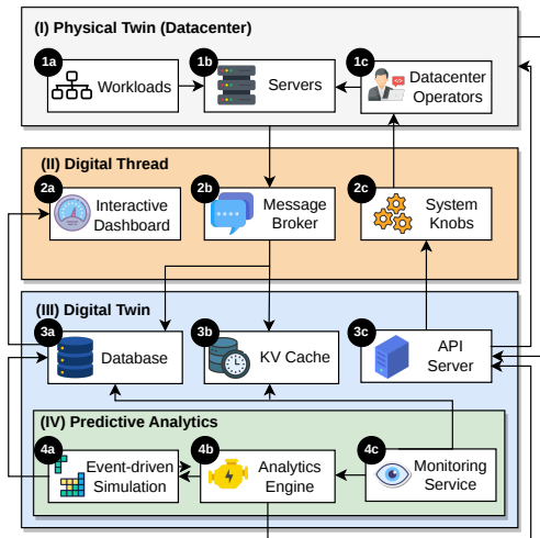
Figure 1.4: The predictive datacenter digital twin architecture.
